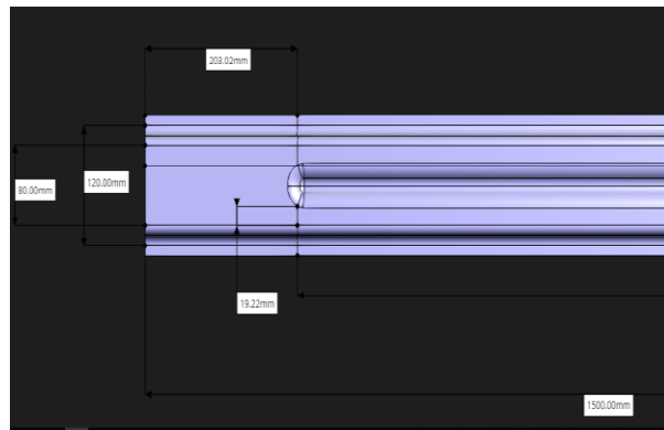
Front view of basic car bumper
