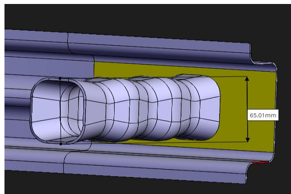
Side view of basic car bumper
