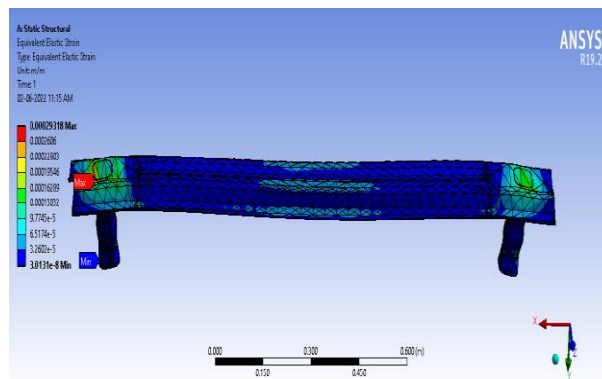
Equivalent elastic strain
