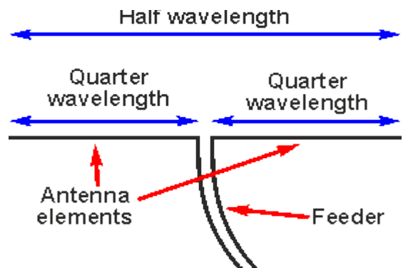
Fig.1. Half Wave dipole center feed. Basically dipole antenna exhibits two terminals or poles through which RF current flows in association with voltage
