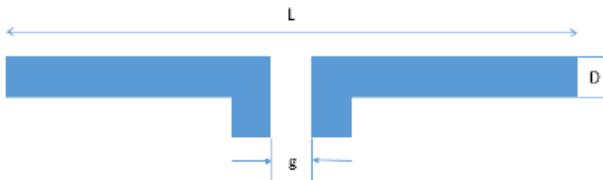
Fig.3. Construction of Half Wave dipole.
