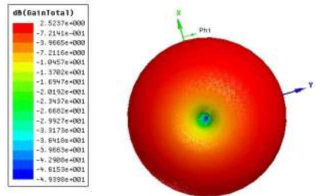
Fig.16. 3D Radiation Pattern shows gain variation.
