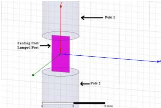
Fig.8. Feeding port or Lumped port
