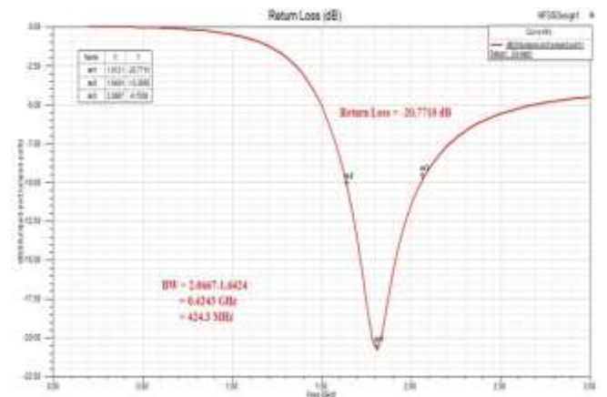
Fig.12. Return Loss curve and Bandwidth for designed half wave dipole antenna.
