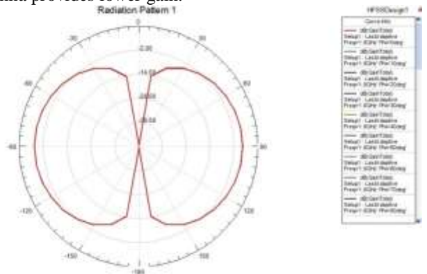
Fig.14. 2D Radiation Pattern for designed half wave dipole antenna.
